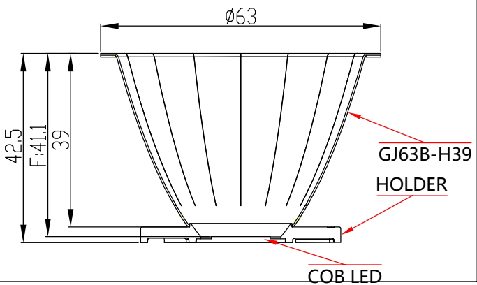
OPTICAL ASSEMBLY DIAGRAM
